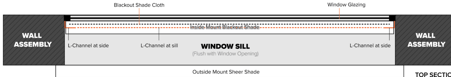
TOP SECTION
