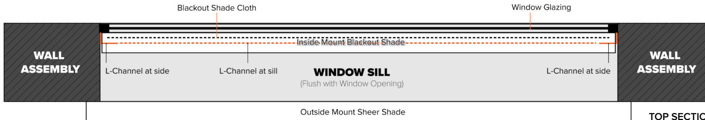
TOP SECTION
