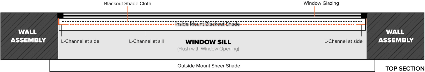
TOP SECTION
