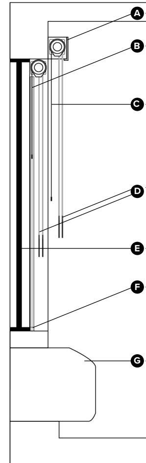
SIDE SECTION
