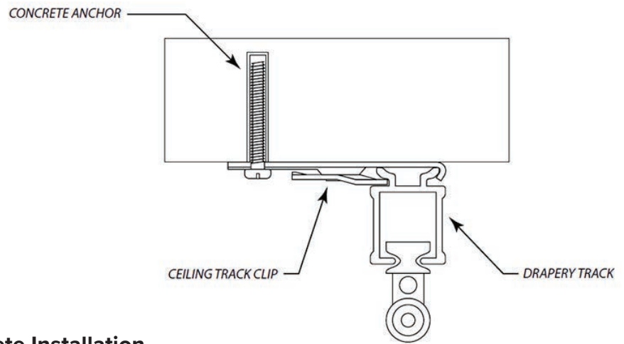
Concrete Installation
