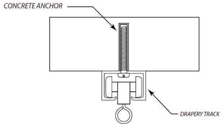
Concrete Installation
