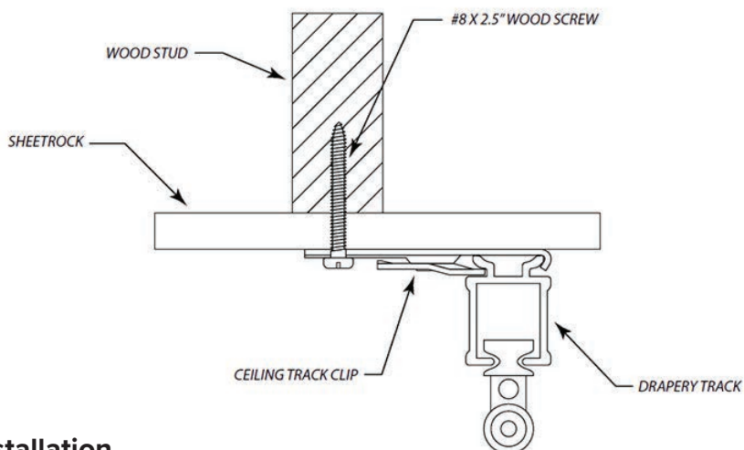
Wood Installation
