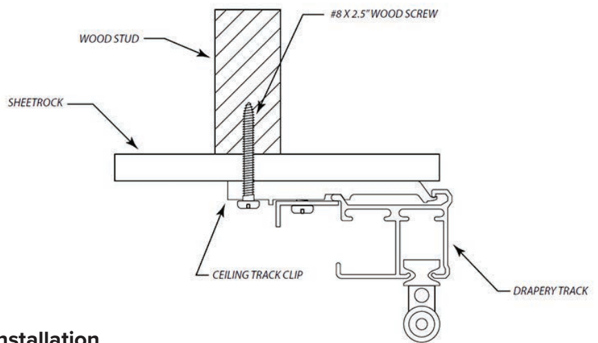
Wood Installation
