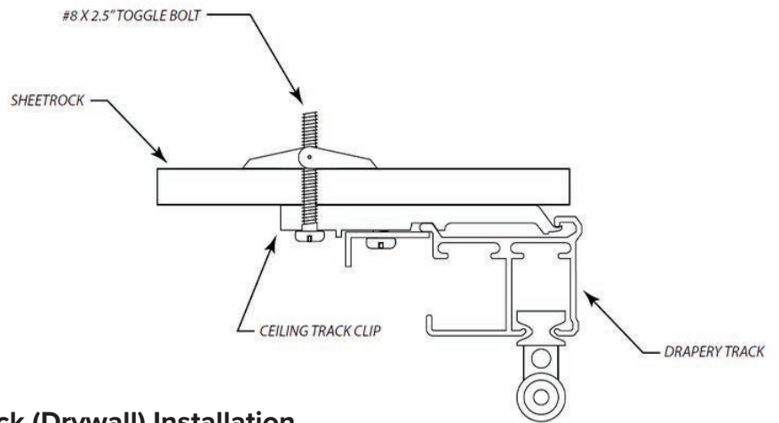
Sheetrock (Drywall) Installation
