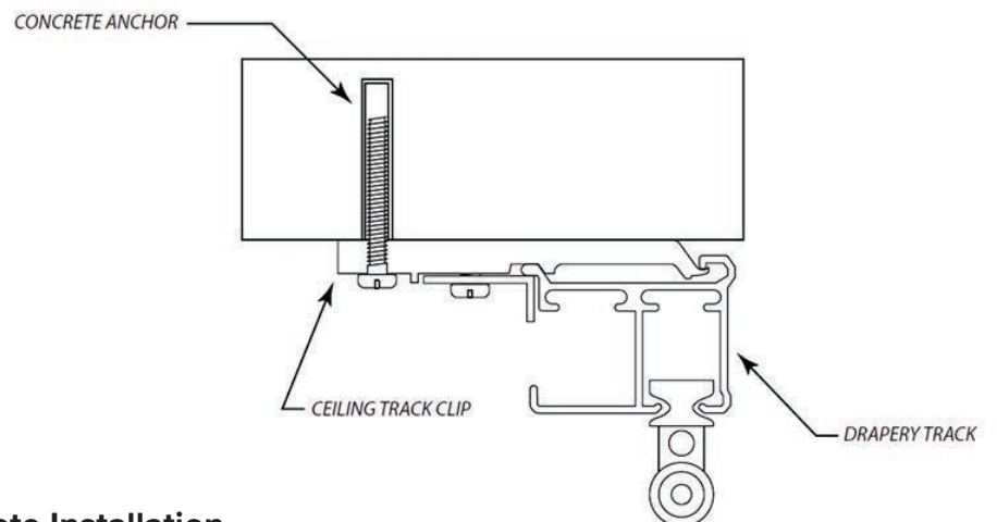
Concrete Installation
