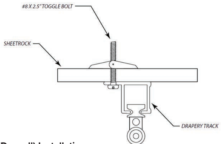
Sheetrock (Drywall) Installation
