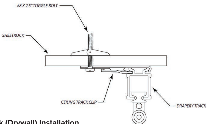
Sheetrock (Drywall) Installation
