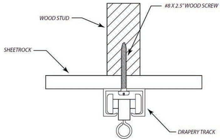
Wood Installation
