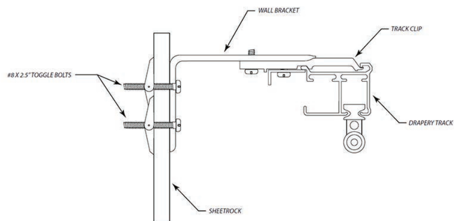
Sheetrock (Drywall) Installation
