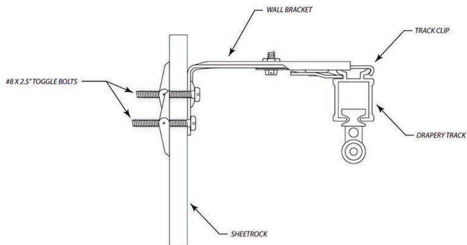
Sheetrock (Drywall) Installation
